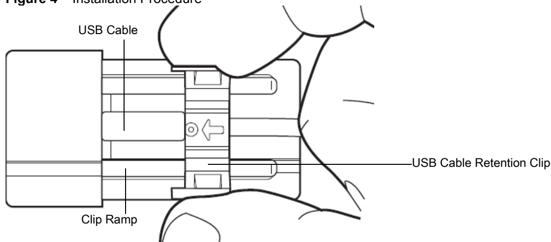
Figure 4 Installation Procedure
