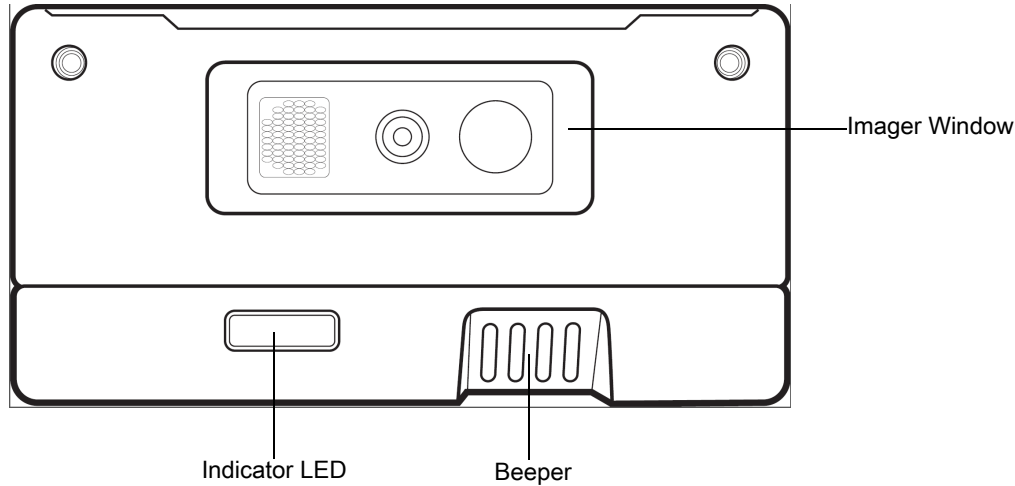
Figure 3 MS4717 Features
